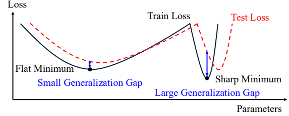
Figure 2. Conceptual 1D Loss Landscape of Flat and Sharp Minima. Figure is reproduced from Keskar et al. [23]. As experimentally shown in Izmailov et al. [18], the test loss landscape tends to be shifted relative to the train loss landscape.
