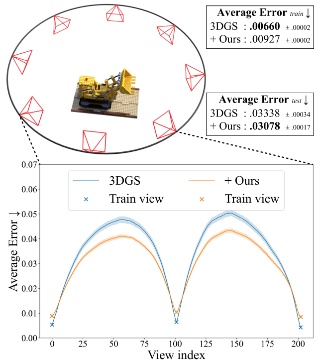
Figure 1. Overview. Our proposed optimization algorithm improves generalization. Given 8 training views rendered from the lego scene in Blender synthetic dataset [40], our method maintains low Average Error [42] across interpolated novel views, whereas the baseline exhibits overfitting. Plots are means and standard deviations over 10 runs.
