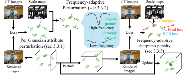
Figure 3. Overview. We first introduce per-Gaussian attribute perturbation as a prerequisite (Sec. 3.3.1). We then propose frequency-adaptive perturbation and sharpness penalty that adjust their magnitude based on local frequency (Secs. 3.3.2 and 3.3.3).
